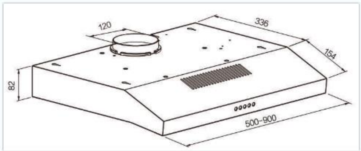
UBSVH60SS Dimensional Drawing
